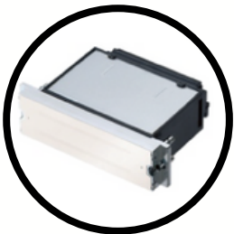
Up to 4 groups of Ricoh Gen6 heads
