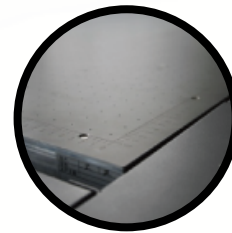
Precise vacuum table with 4 selectable zones, media alignment pins and blowing function
